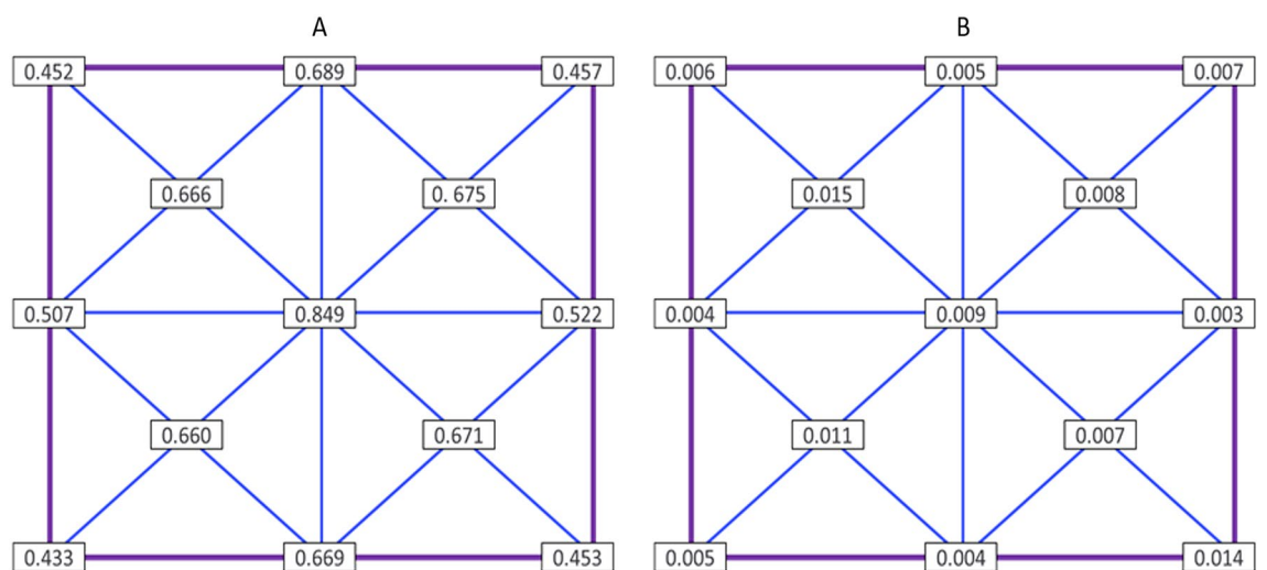
Figure 3. Average values of irradiance (a) and standard deviations (b) obtained from testing three lamps at given points within the UV-C device ( \text{mW}/\text{cm}^2 ).
