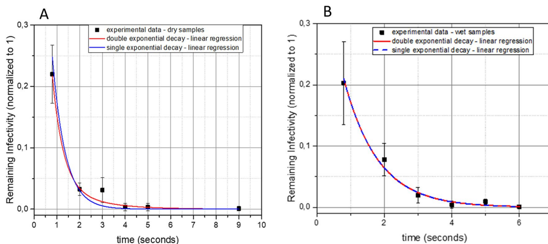
Figure 1. Reduction in infectivity of SARS-CoV-2 after exposure to UV-C irradiation. The virus was exposed to UV-C as dried droplets (A) or wet droplets (B). Each set of data (dry samples and wet samples) shows a decrease of the remaining infectivity as a function of time, normalized to 1. Blue lines indicate single exponential decay functions while red lines indicate double exponential decay functions.
